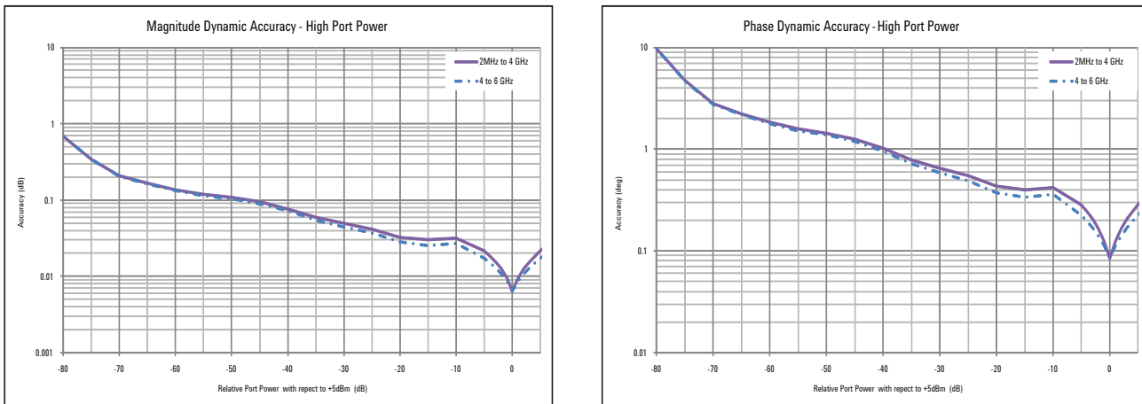
Figure 10: Dynamic accuracy (specification)
